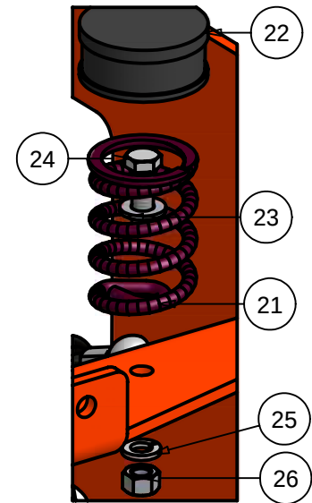
DETAIL A
